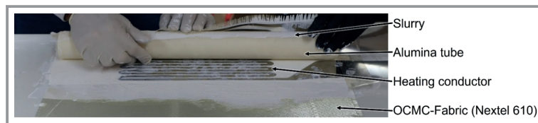
Figure 2. Components of an electrical hybrid OCMC tube with embedded electrical heater.
